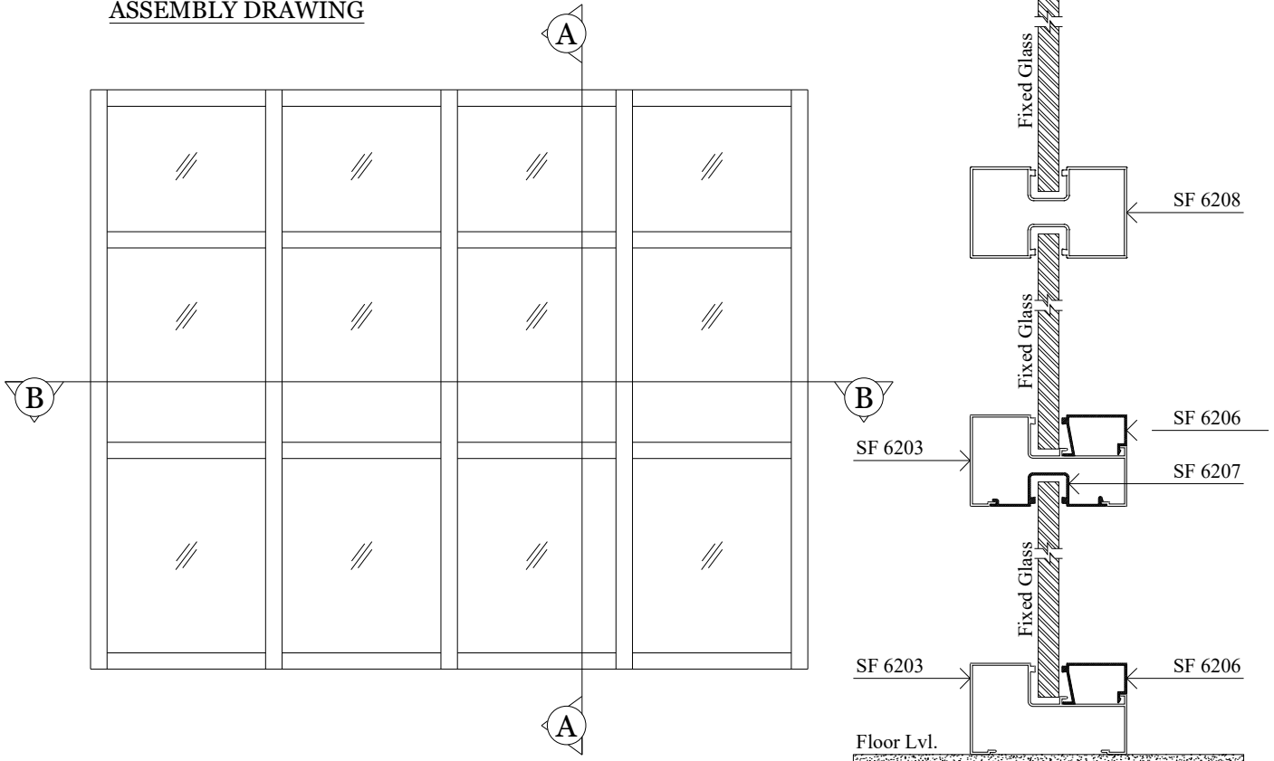
ASSEMBLY DRAWING
