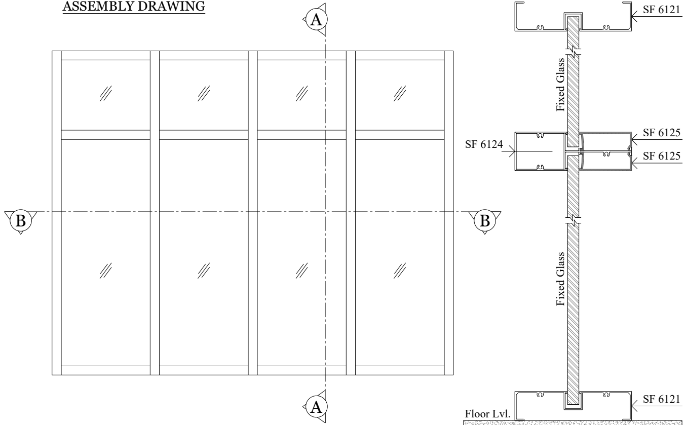
ASSEMBLY DRAWING
