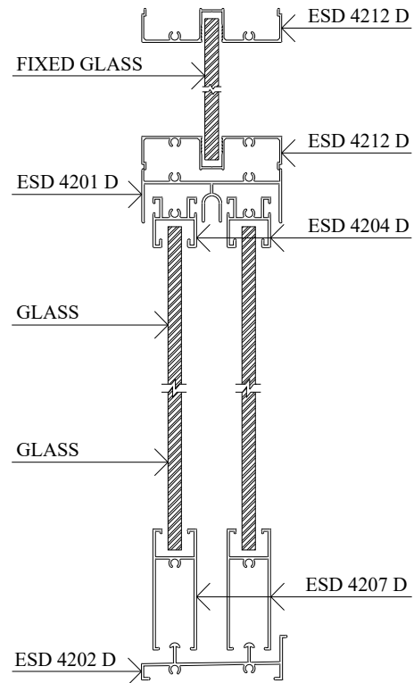
SECTION VIEW A - A
