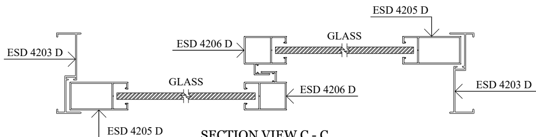
SECTION VIEW C - C
