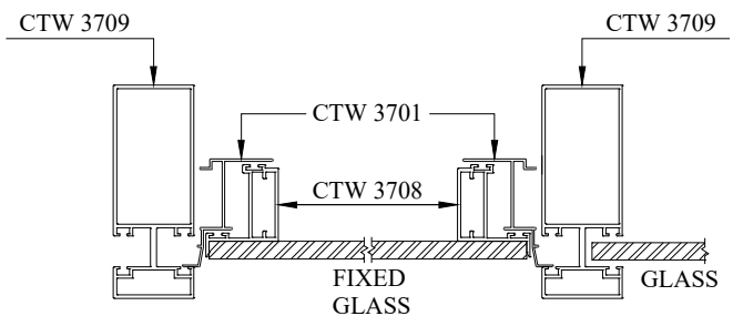
SECTION VIEW C - C
